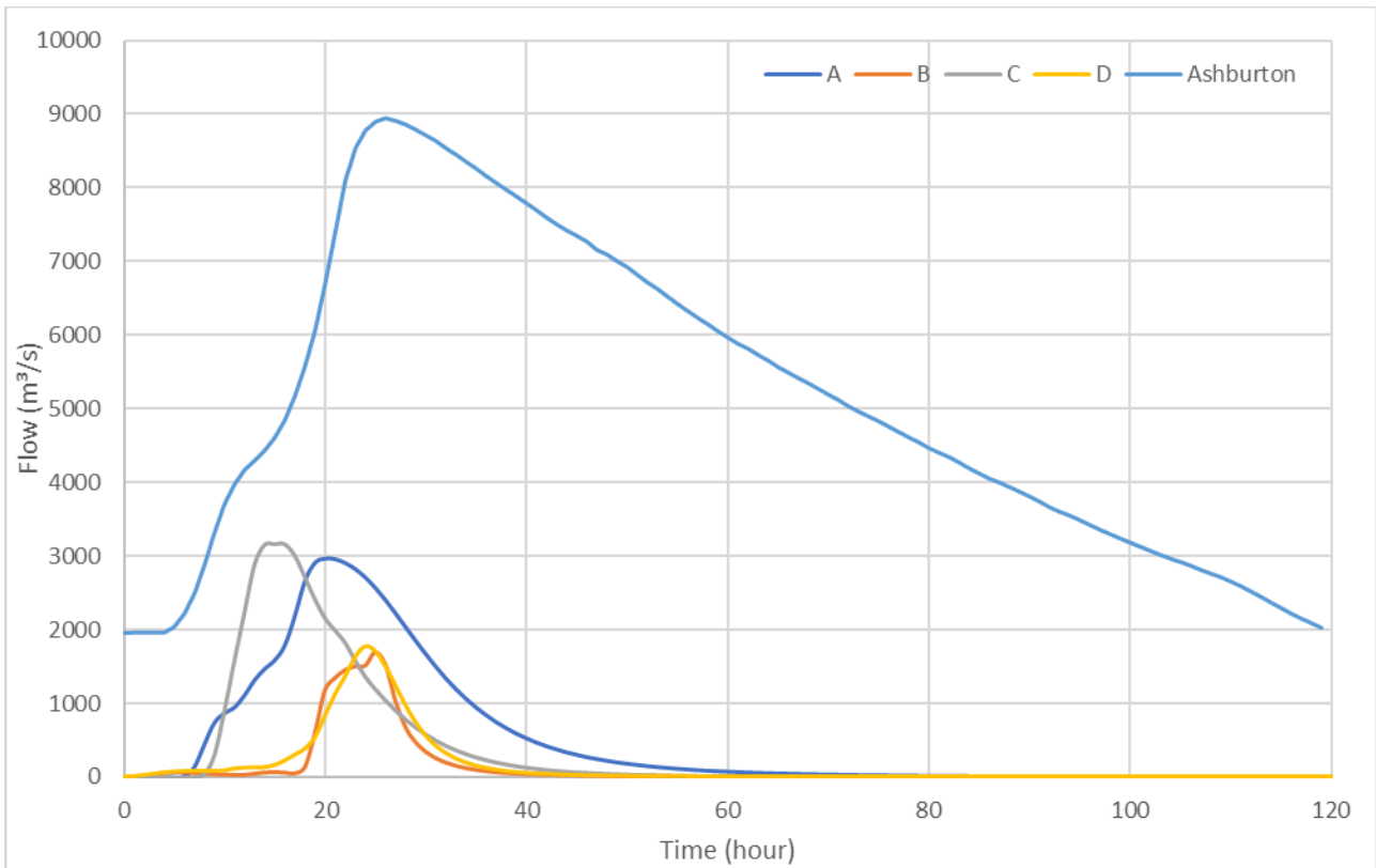
FIGURE 7-12 INFLOW HYDROGRAPHS FOR THE 2% AEP EVENT
