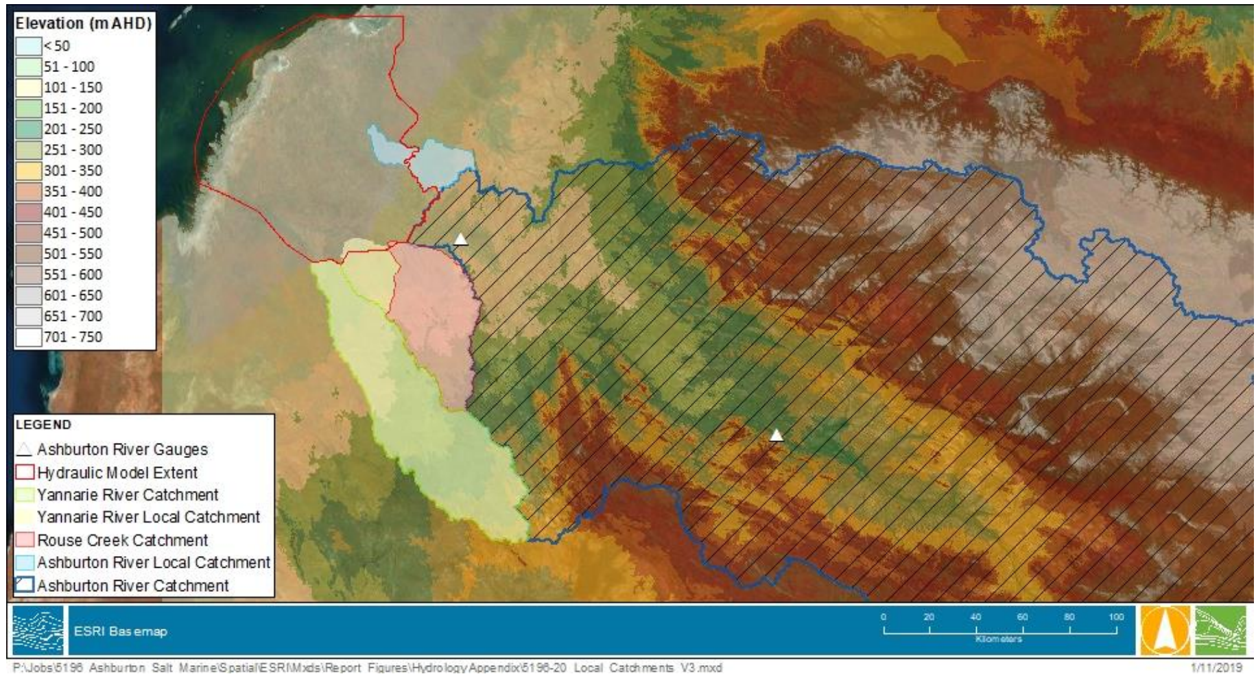
FIGURE 3-2 LOCAL CATCHMENT LOCATIONS
